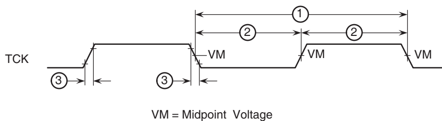
Figure 4-14. JTAG Clock Input Timing Diagram
