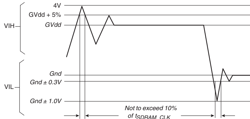
Figure 3-2. Overshoot/Undershoot Voltage
