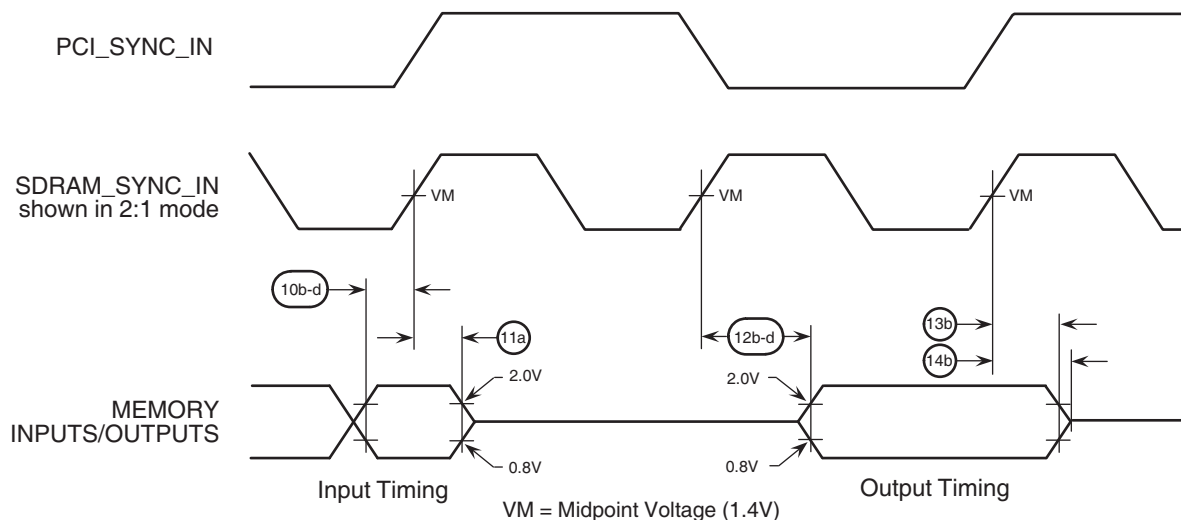
Figure 4-3. Input – Output Timing Diagram Referenced to SDRAM_SYNC_IN
