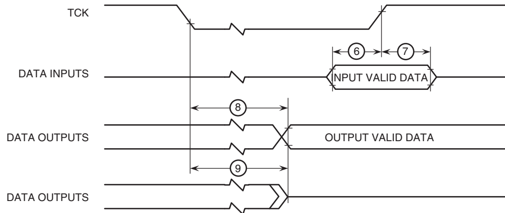
Figure 4-16. JTAG Boundary Scan Timing Diagram
